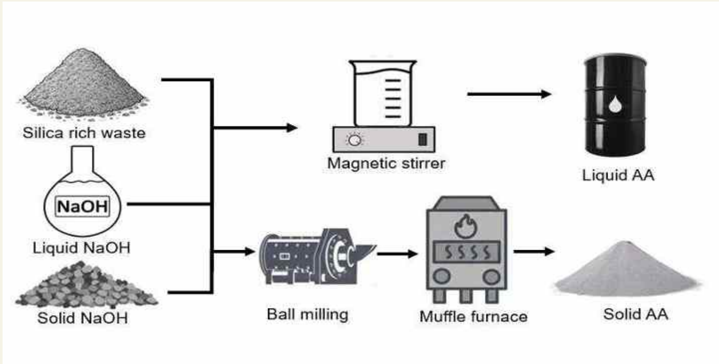
Figure 1. Schematic illustration of alternative AA production
