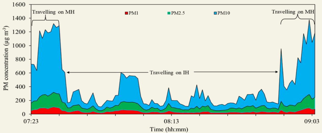
Fig. 1 Temporal variation of dumper in-cabin PM concentration (MH- Main haul road, IH- Internal haul road)
